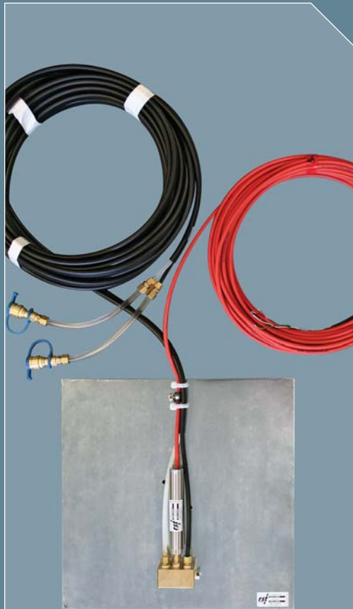
Typical installation of a Vibrating Wire Liquid Settlement System.
